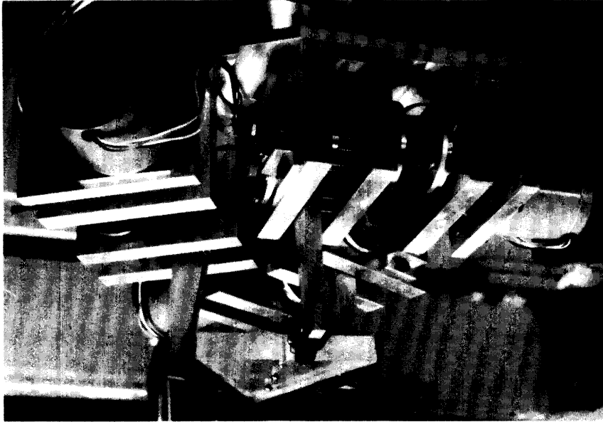
Figure 4. A three-fingered hand designed by Haruhiko Asada to grasp planar objects stably and to execute incremental compliant motions. Each single degree-of-freedom finger is actuated by a stepping motor, and contains a passive leaf spring.
