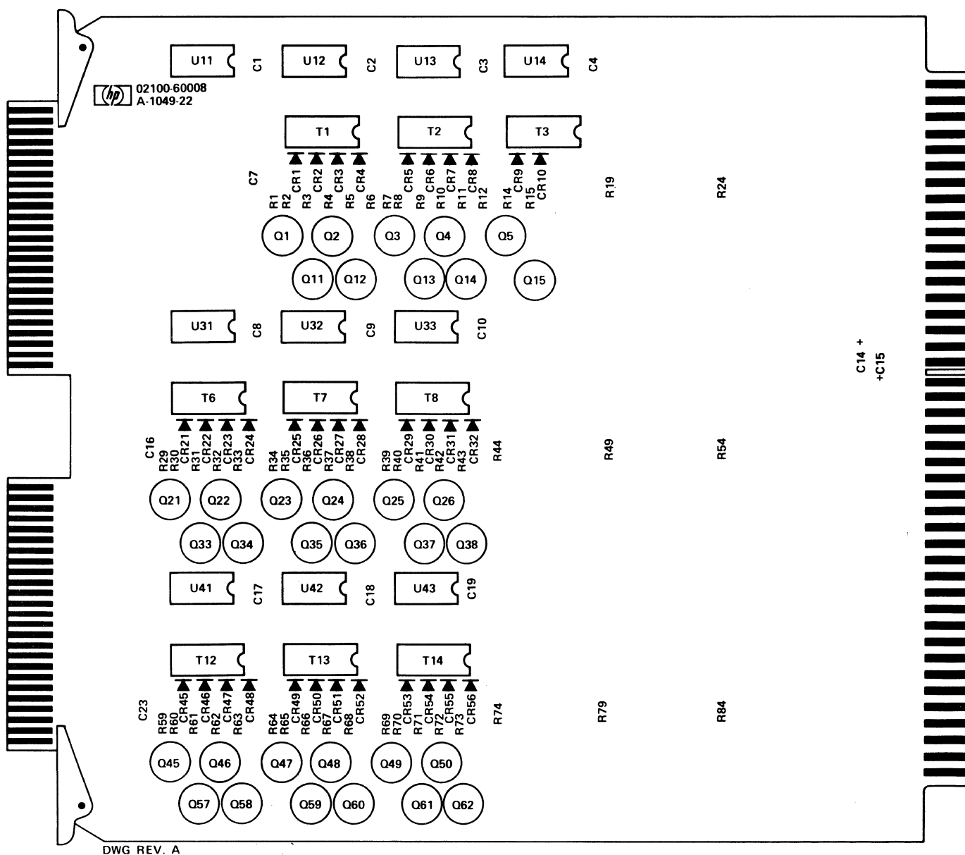
Figure 2-15. A105 Inhibit Driver Card (8K), Parts Location Diagram
