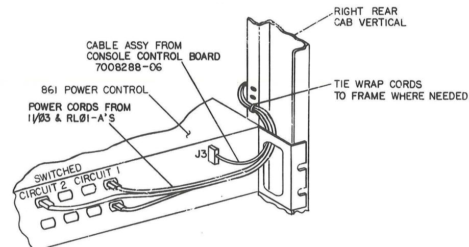
VIEW A-A PART OF FIGURE-1 (REAR VIEW)
