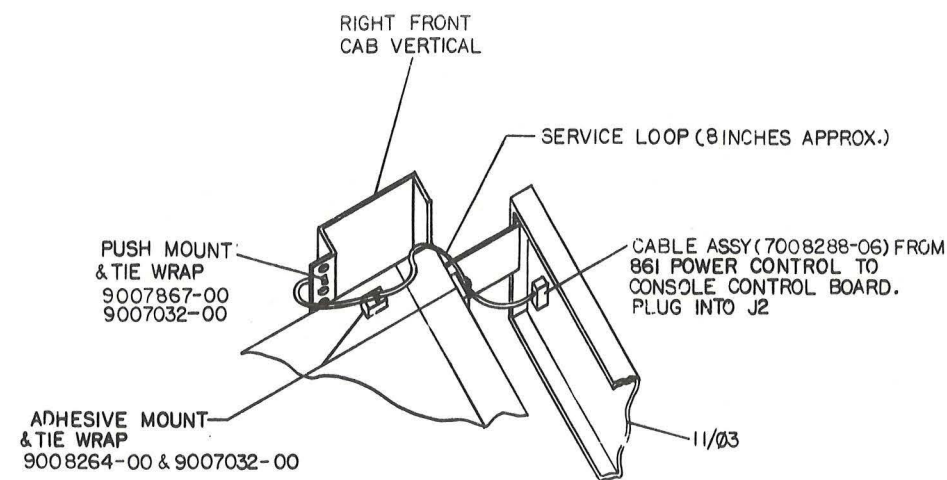
DETAIL 'A' PART OF FIGURE-1 (TOP VIEW)
