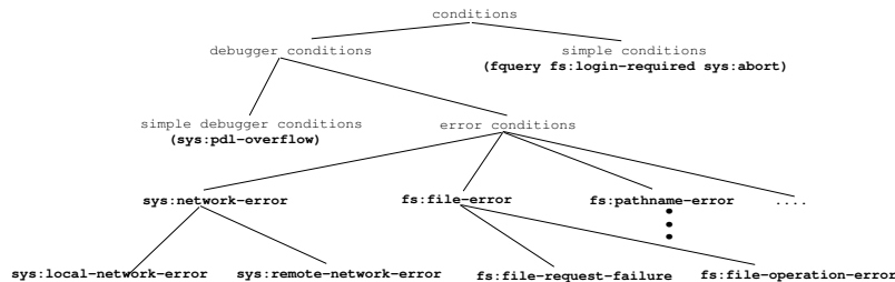
Figure 22. Condition Flavor Hierarchy
