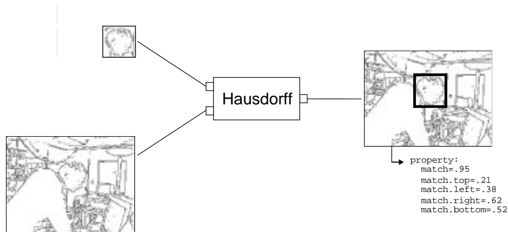
Figure 4-6: VsHausdorff
