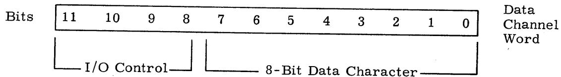
Figure 3-1. Output Word Format
