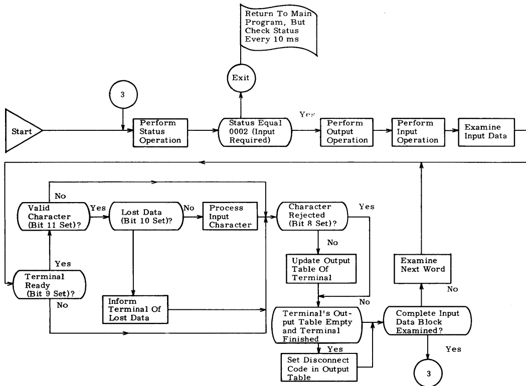
Figure 3-4. Sample Multiplexer Servicing Routine
