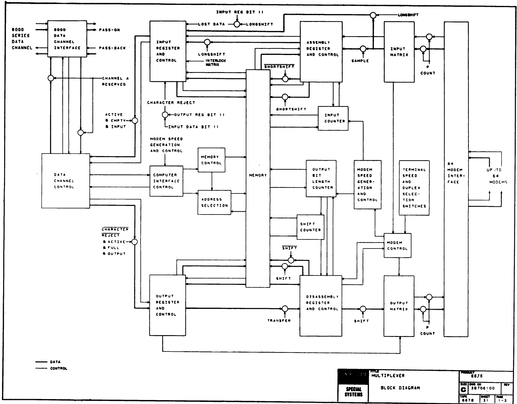
Figure 2-1. Multiplexer Block Diagram
