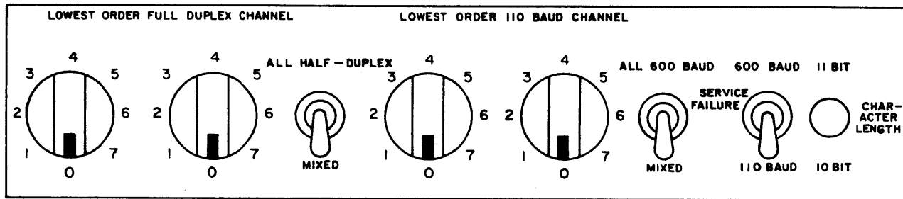
Figure 2-3. 6676-A Switch Panel
