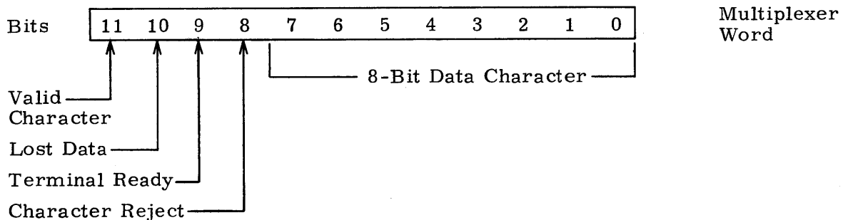
Figure 3-2. Input Word Format
